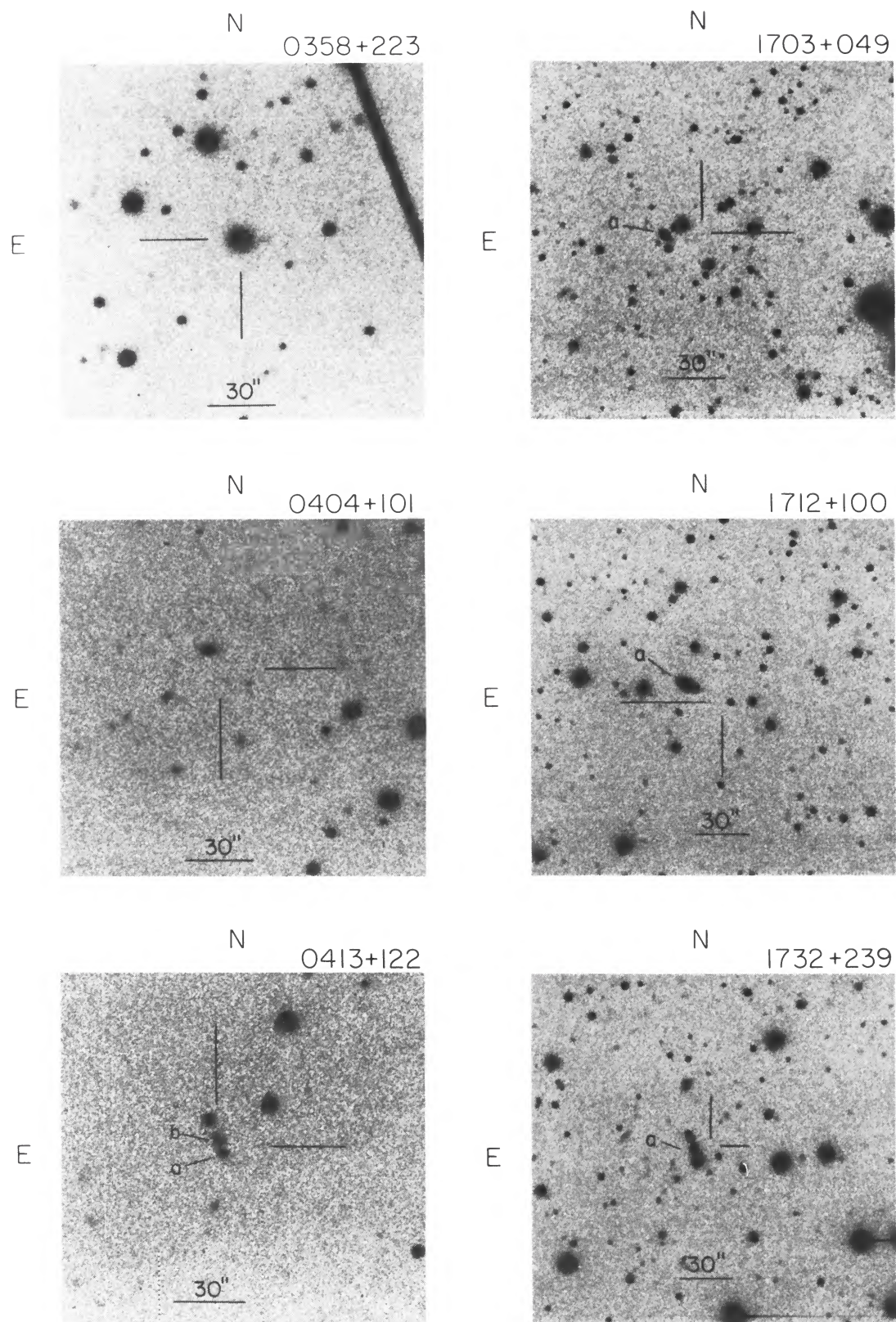
FIG. 1.—The r images of 0358+223, 0404+101, 0413+122, 1703+049, 1712+100, and 1732+239 obtained with the 5 m telescope. The IRAS position is indicated, and the identified galaxy is either indicated as object a or is the only object close to the IRAS position.
