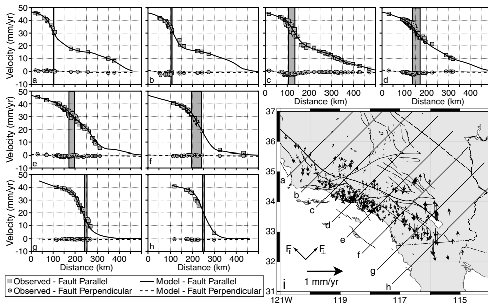
Figure 5. (a–h) SCEC 3 Observed versus interpolated surface velocities (used in strain rate calculations) with 500 km of cross-sections through southern California. (i) Cross-section locations and misfit between observed and interpolated velocities.
